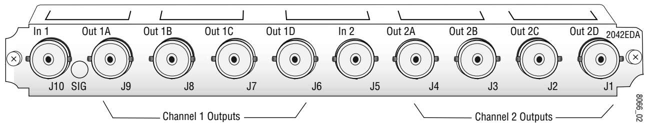
Figure 5. 2042EDA Input/Output Connectors (with overlay installed)
