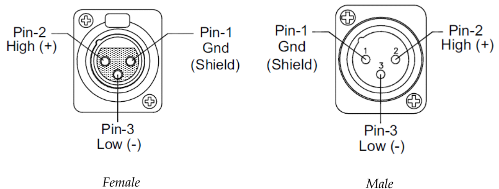
Figure 1–6 XLR Pin-Outs
